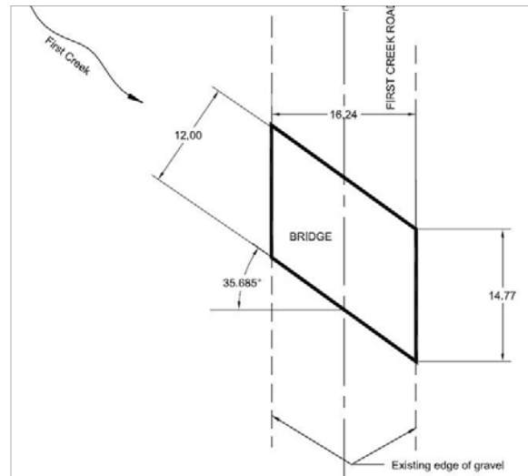
Bridge Detail
