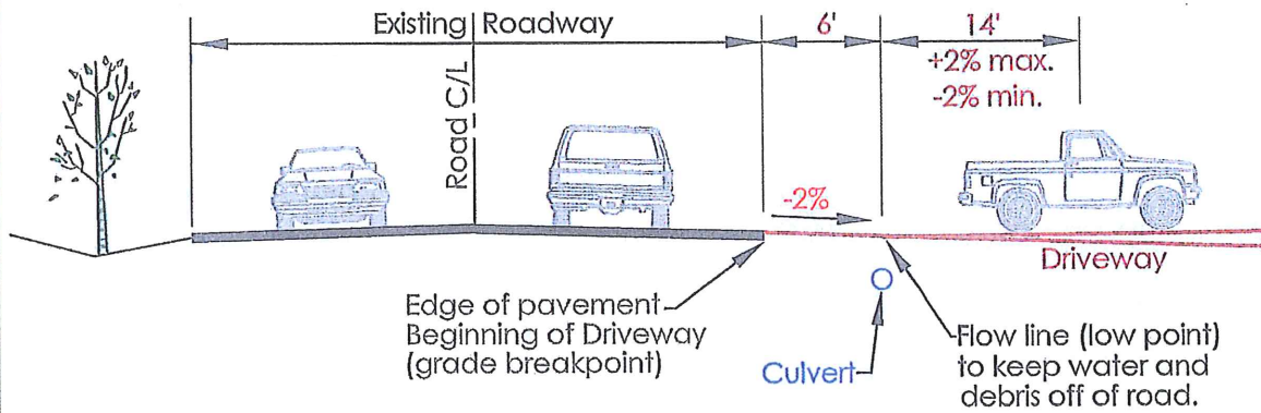
TYPICAL SECTION
