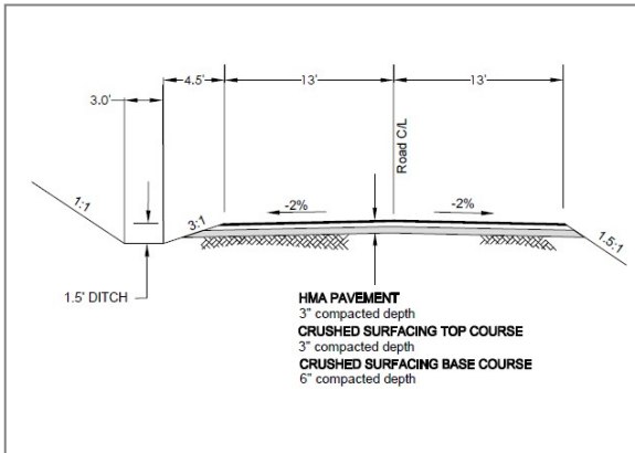
Project Typical Section
